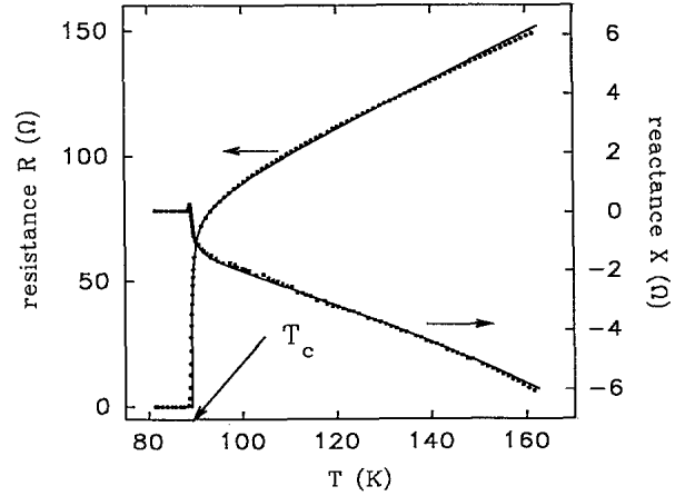
FIG. 4. A typical result for the T dependence of the resistance R at a frequency of 60 kHz. The three samples we measured gave essentially the same results. Drawn curves are a fit with a model explained in the text.
