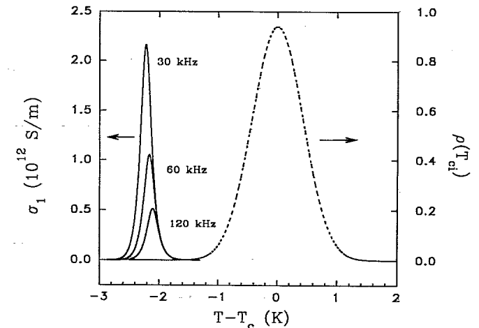
FIG. 2. Peak in the real part of the conductivity \sigma_1 , obtained from the linear-chain, Gaussian broadened two-fluid model, at frequencies of 30, 60, and 120 kHz. The Gaussian distribution \rho(T_{ci}) with a full width at half height of 1 K is displayed in the figure also. Parameters are the same as in Fig. 1.
